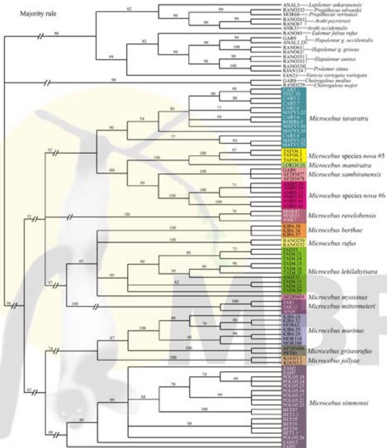
Appendix II(d). Fifty percent majority-rule consensus phylogenetic tree from the Bayesian analysis derived from the D-loop sequence data from 77 Microcebus individuals with 18 out-group taxa reconstructed using the program MrBayes. Branches without posterior probability values (PP) are supported by less than 50% of the sampled trees.
