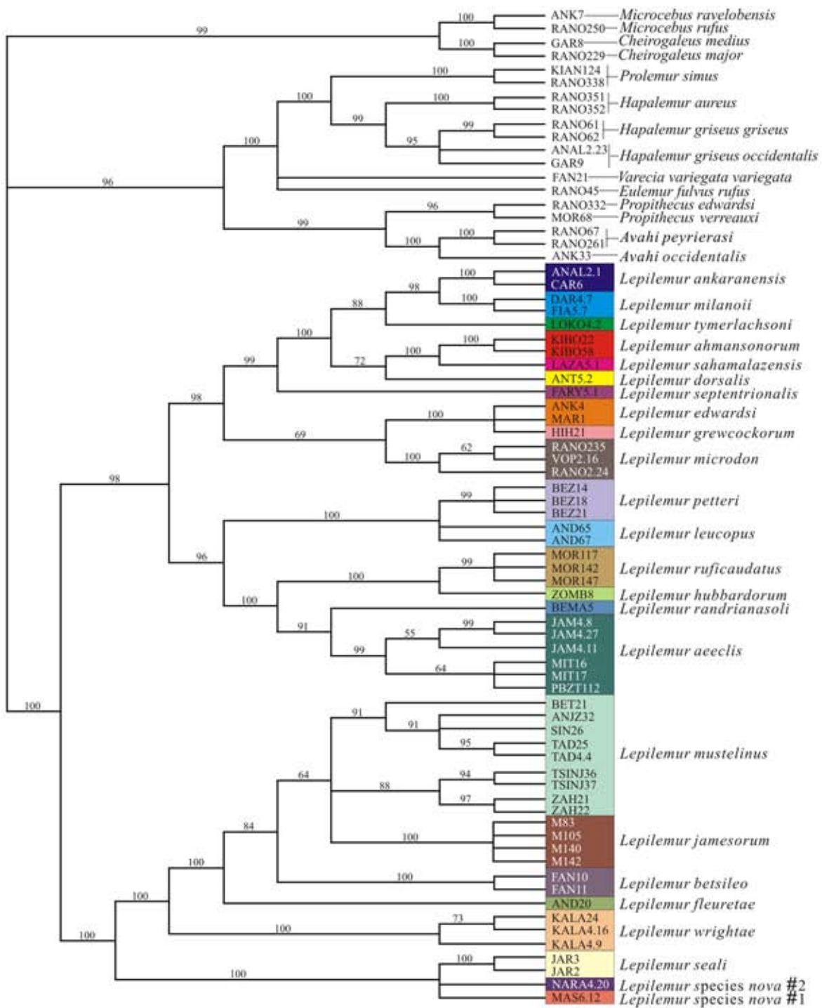
Appendix II(r). Fifty percent majority-rule consensus phylogenetic tree from the Bayesian analysis derived from the 12S rRNA sequence data from 55 haplotypes from the 216 Lepilemur individuals with 19 out-group taxa reconstructed using the program MrBayes. Branches without posterior probability values (PP) are supported by less than 50% of the sampled trees.
