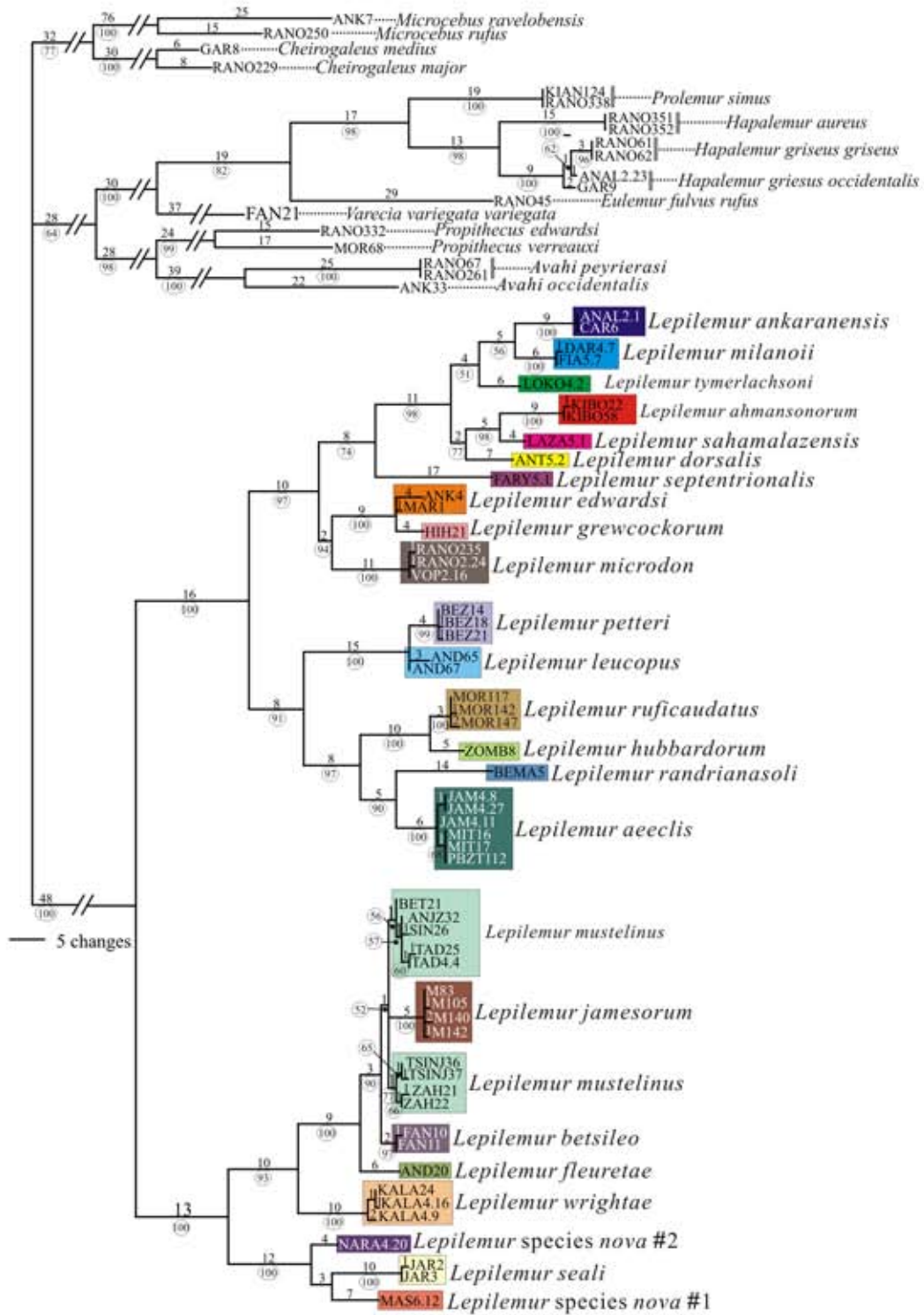
Appendix II(o). Neighbor-joining phylogram derived from the 12S rRNA sequence data from 55 haplotypes from the 216 Lepilemur individuals with 19 out-group taxa. Values above branches indicate number of changes between nodes. Values within circles along the branches indicate support of bootstrap pseudoreplicates.
