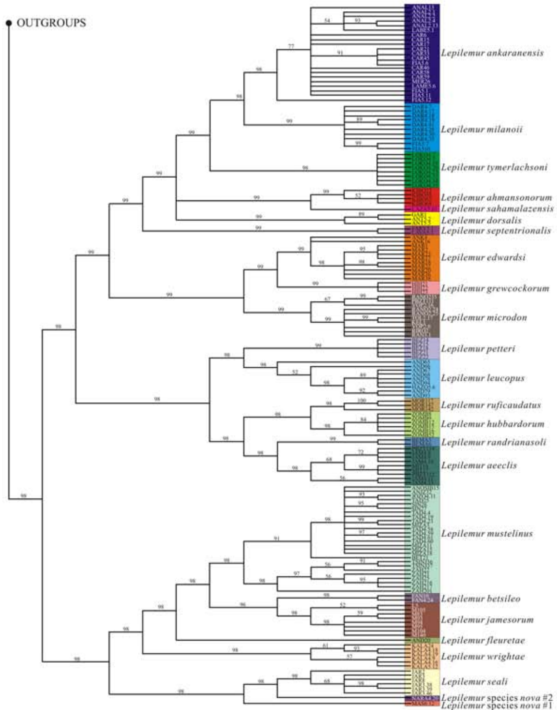
Appendix II(n). Fifty percent majority-rule consensus phylogenetic tree from the Bayesian analysis derived from the PAST sequence data from 158 haplotypes from the 216 Lepilemur individuals with 19 out-group taxa reconstructed using the program MrBayes. Branches without posterior probability values (PP) are supported by less than 50% of the sampled trees.
